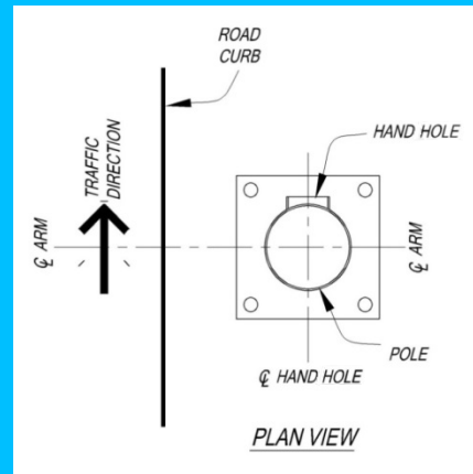
Figure C5.6.6.1-1—Recommended Orientation of a Hand Hole
