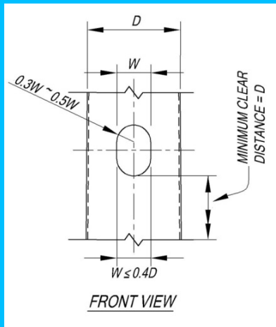
Figure 5.6.6.1-1—Details of Unreinforced Holes and Cutouts
