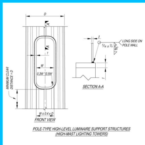
Figure 5.6.1-3—Details of Reinforced Holes and Cutouts for High-Mast Poles
